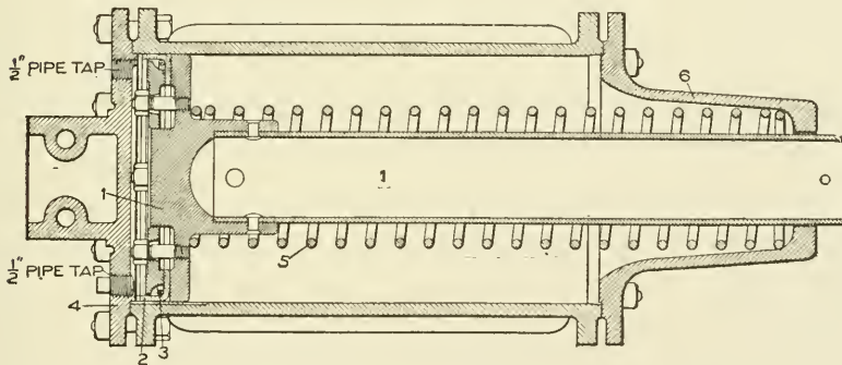
Fig. 92. Brake Cylinder of Hollow-Rod Type
